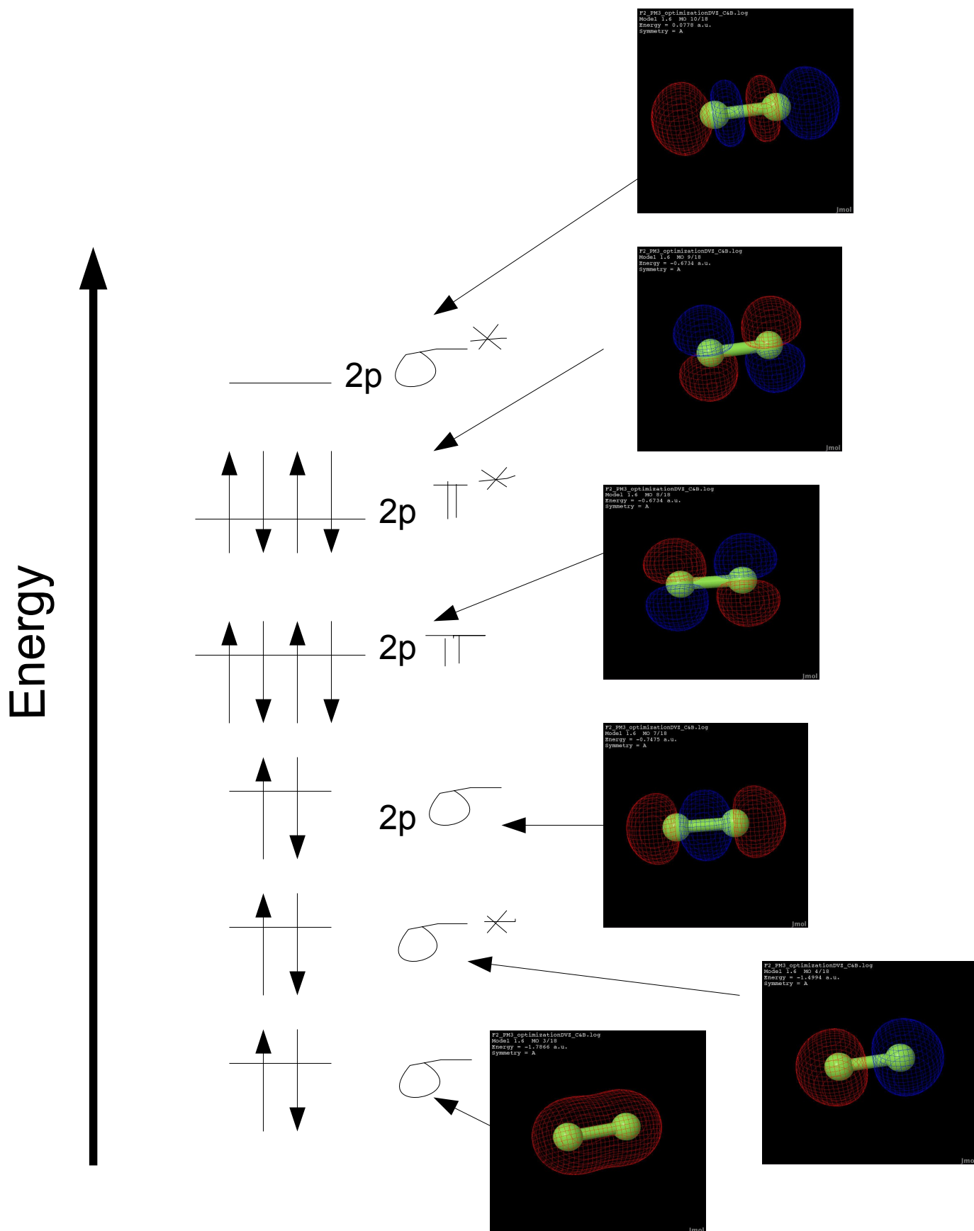
Figure 1: Valence Energy Level Diagram of F 2
